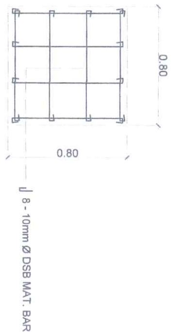
DRAINAGE COVER DETAIL
